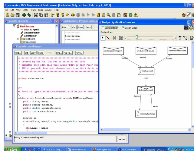
Figure 3. Screenshot of JACK Integrated Development Environment (IDE)
